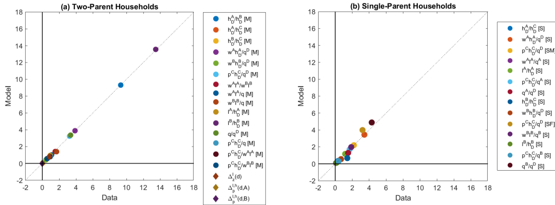
Figure A.2: Model Fit of Estimation with Quasi-Experimental Moments
